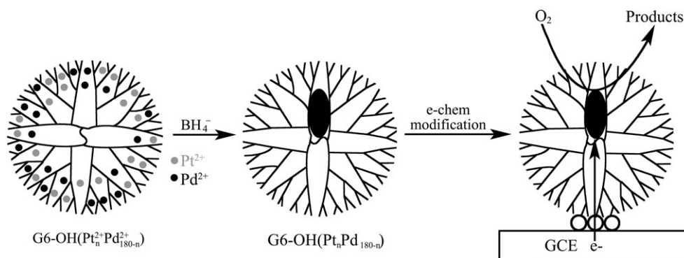
Scheme 2 Electrocatalytic O_2 reduction at glassy carbon electrodes (GCEs) modified with PdPt DENs.
